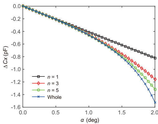
Fig. 5 Comparison of differential capacitances as functions of \alpha between calculation results ( n = 1, 3, 5 ) and numerical integration ( R_i , R_o , h_o , and \theta_0 are 2 mm, 5 mm, 200 \mu\text{m} , and 43^\circ , respectively)
